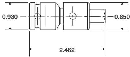
1/2" Adapter
